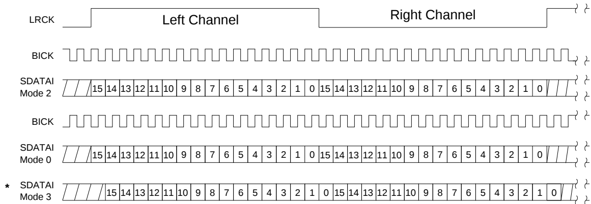
Figure 6. Digital Input Formats 0, 2 and 3 with 16 BICK Periods
